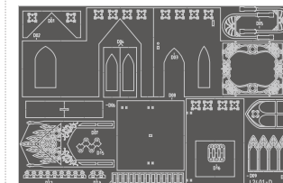
Board D Plywood(Dark gray) 30*20*0.2cm(1 piece)
