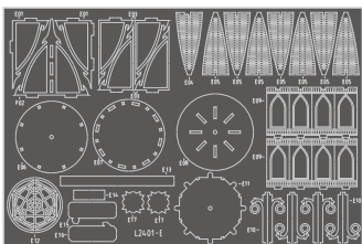
Board E Plywood(Dark gray) 30*20*0.2cm(1 piece)
