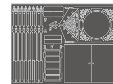
Board G Plywood(Dark gray) 20*15*0.2cm(1 piece)
