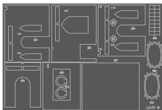
Board B Plywood(Dark gray) 30*20*0.3cm(1 piece)
